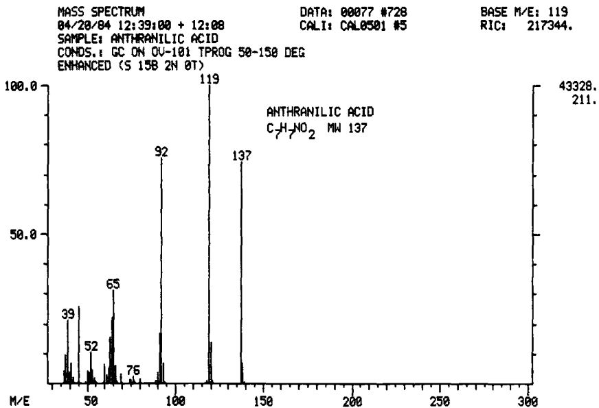
FIG. 2—Normalized 80 eV, EI, mass spectra of Compounds I through IX.
